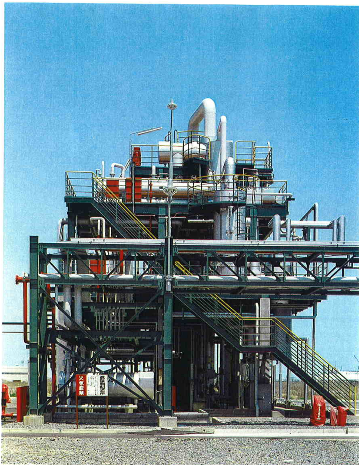
Above shown is the Yokkaichi Plant which produces an aromatic resin PETCOAL by the continuous polymerization of C_9 fractions derived from the steam-cracking of petroleum naphtha. The production capacity of PETCOAL is 15,000 tonnes per year.
