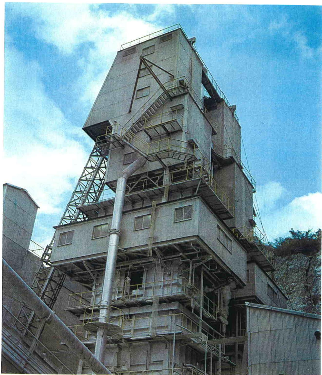
A view of the 150 t/day Maerz type calcining kiln at Matsukawa factory of Tohoku Tekkosa Co., Ltd. The automatic kiln operated by the central controlling system features a greater fuel economy.
