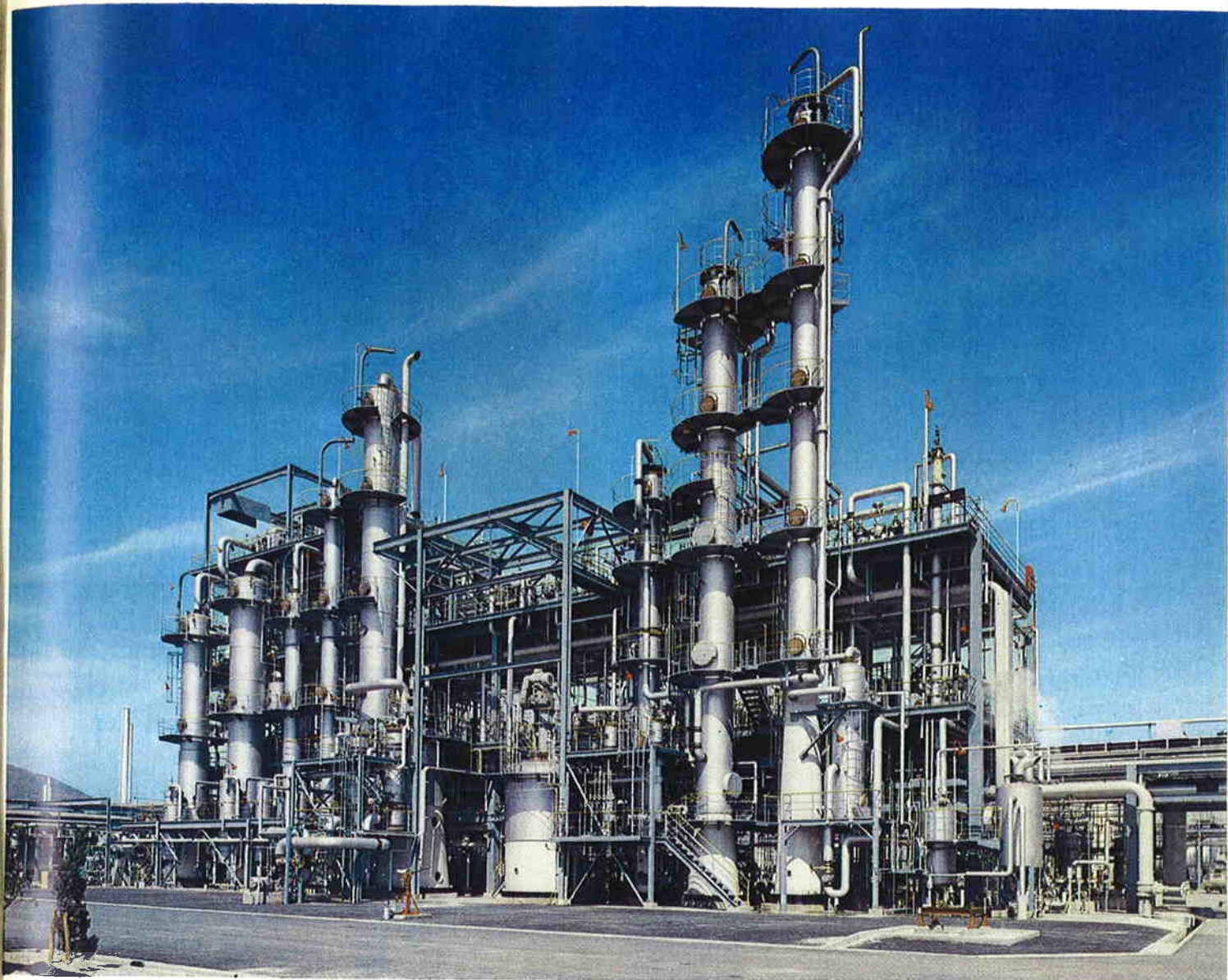
Chloroprene Monomer Plant at Shinnanyo-shi, Yamaguchi, working on since April, 1971, produces 12,000 tons/year of monomer by the butadiene process.
