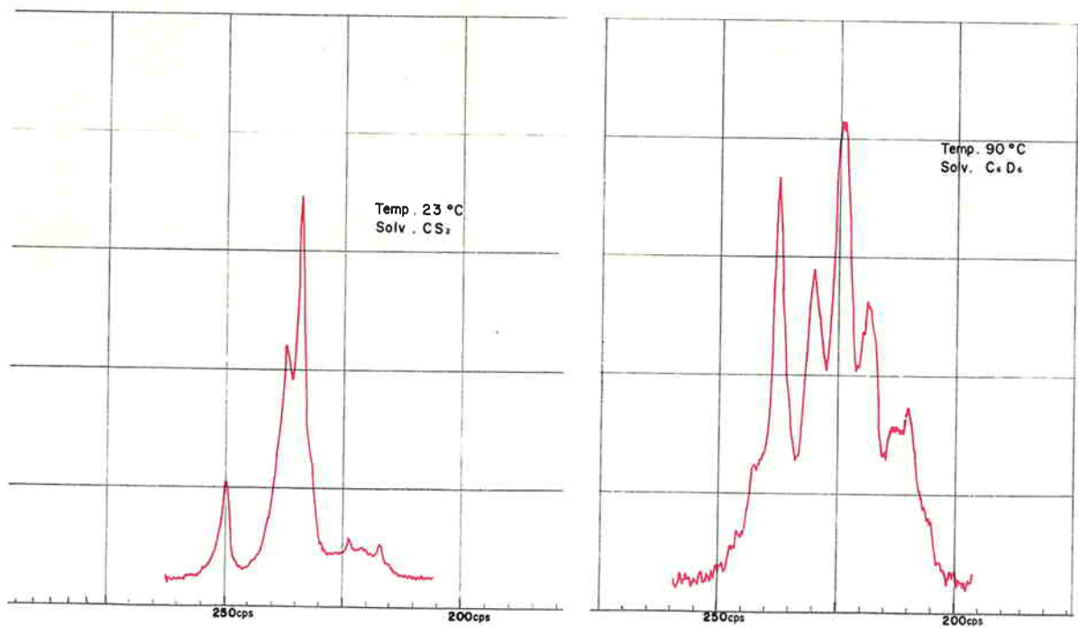
NMR Spectra of Polychloroprene
