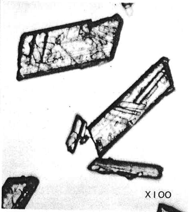
Micro-Photographs of Sodium Bicarbonate Crystals Made in TOYO SODA Plant
