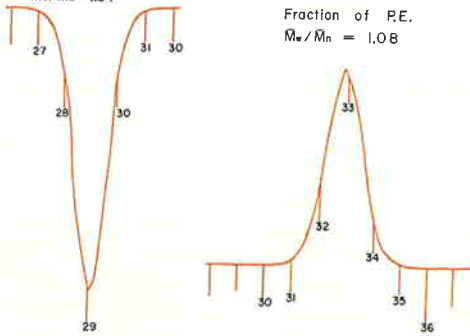
GPC Pattern of Fractionated Polyethylene
